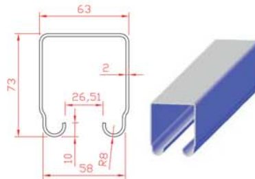
Guia superior
